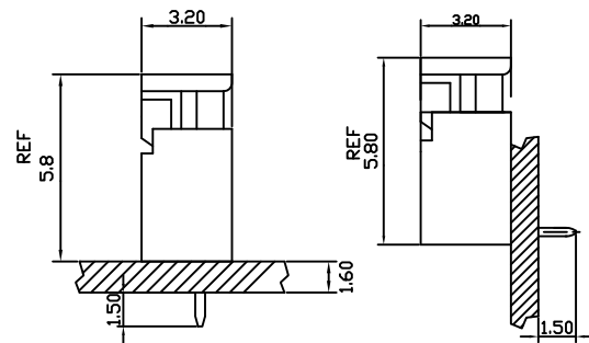
DIP TYPE
